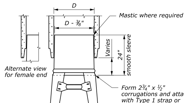
FOR ALL SIZES OF CONCRETE ROUND OR PIPE ARCHES
