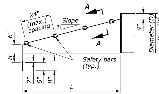
ELEVATION PARALLEL DRAINAGE END SECTION
