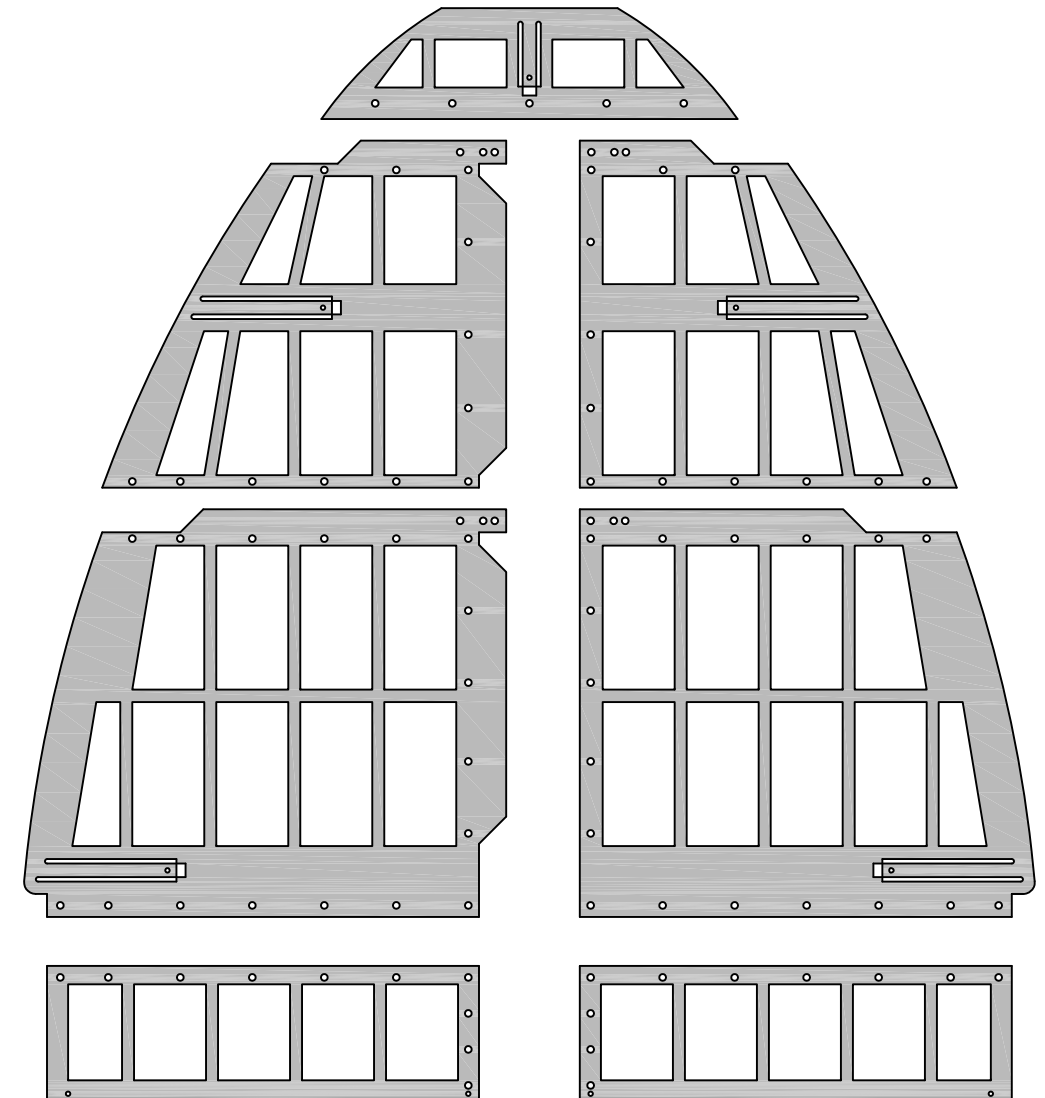
TYPICAL TRASH GUARD (Five Piece Top) (Two Piece Front)
