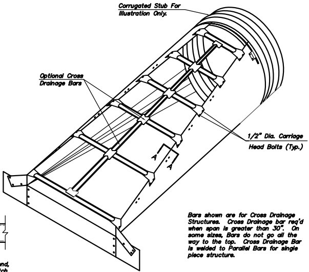
48" CROSS DRAINAGE STRUCTURE 6:1 SLOPE
