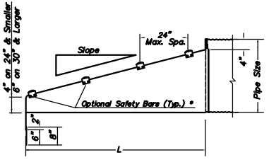
SIDE ELEVATION OF PARALLEL DRAINAGE STRUCTURE
