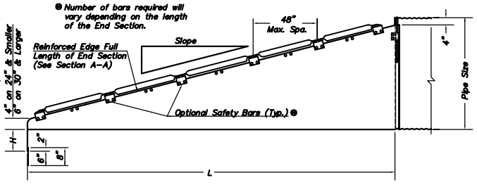
SIDE ELEVATION FOR CROSS DRAINAGE STRUCTURE
