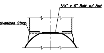
TYPE #1 CONNECTOR DETAIL
