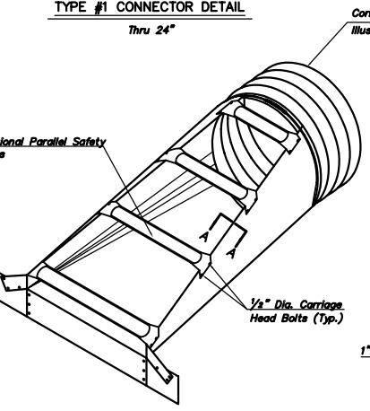
24" PARALLEL DRAINAGE STRUCTURE 6:1 SLOPE
